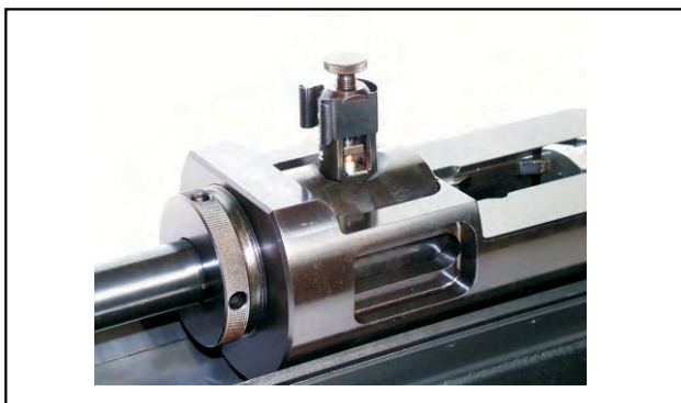
PRESSURE BALLISTIC BARREL WITH PRESSURE CRUSHER GAUGE
